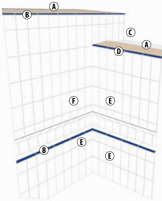
DETAIL 2 | JUMP LEVEL/POOL EDGE
